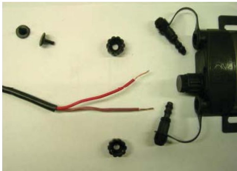
Photo 12 inserting the prepared, stripped solar panel cable into the power-bus plugs at one end of the SFM1
